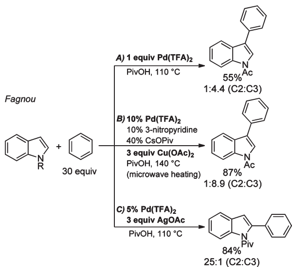
SCHEME 5. Oxidative Cross-Coupling of Indoles and Benzene with Stoichiometric Transition-Metal Oxidants 26
