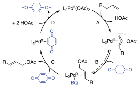
SCHEME 3. Proposed Mechanism for Pd-Catalyzed Allylic Acetoxylation Using BQ as the Oxidant
