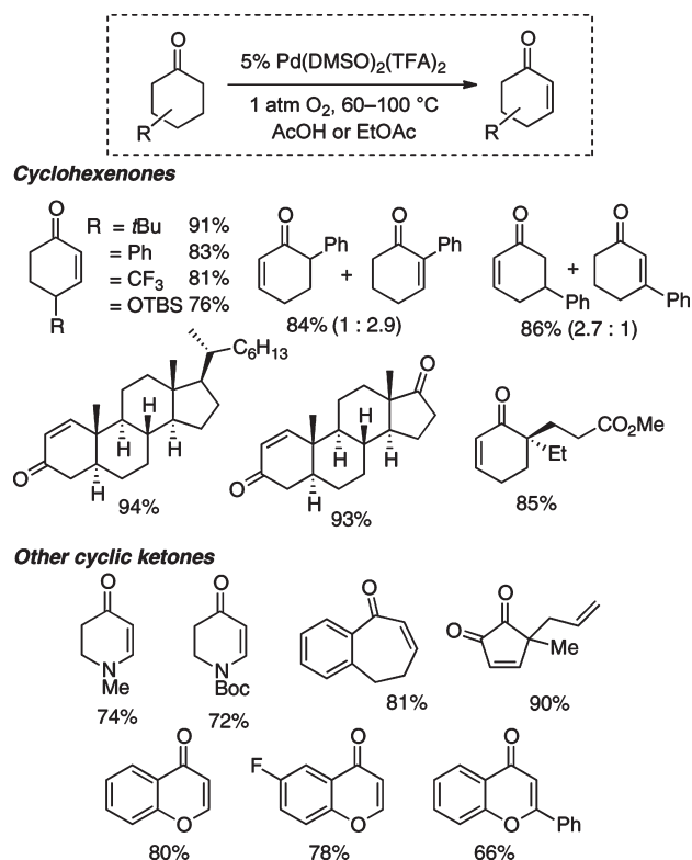
CHART 6. Enones Prepared via Dehydrogenation of Cycloketone Derivatives
