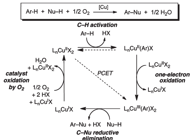
SCHEME 10. Stepwise Mechanism for Cu-Catalyzed Aerobic C–H Oxidation
