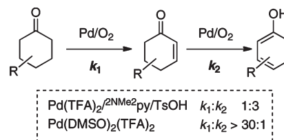
SCHEME 8. Aerobic Dehydrogenation Provides Access to Phenols or Cyclohexenones
