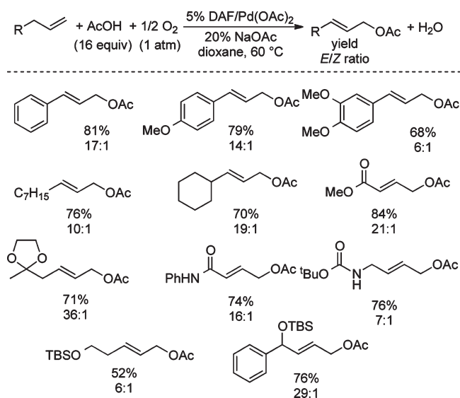
CHART 2. Aerobic Allylic Acetoxylation of Terminal Alkenes
