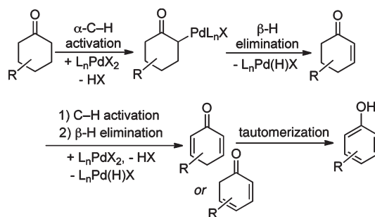
SCHEME 7. Stepwise Sequence of Pd II -Mediated Dehydrogenation of Cyclohexanones
