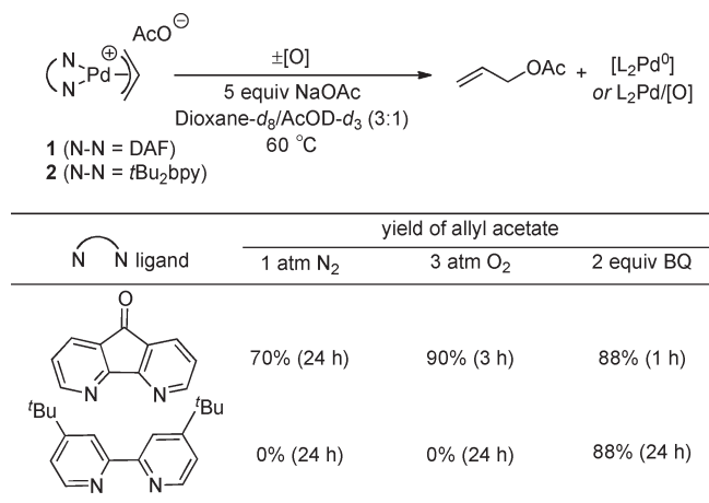
FIGURE 1. Ligand effects on stoichiometric acetoxylation of \pi -allyl-Pd complexes.
