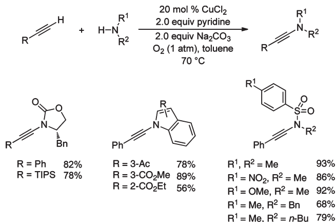
SCHEME 12. Aerobic Copper-Catalyzed Synthesis of Ynamides from Terminal Alkynes
