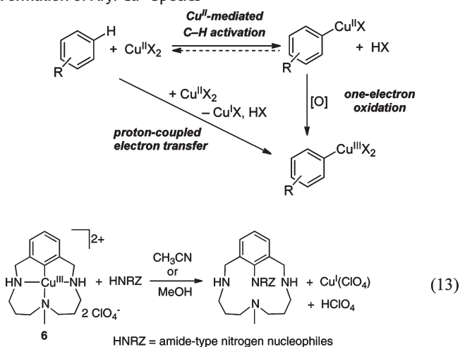
SCHEME 9. Possible Mechanisms for Cu II -Mediated C–H Activation and Formation of Aryl-Cu III Species
