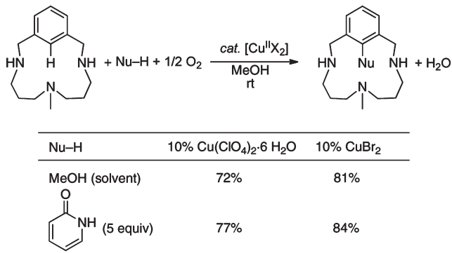
SCHEME 11. Oxidative Functionalization of 6 Catalyzed by Cu II
