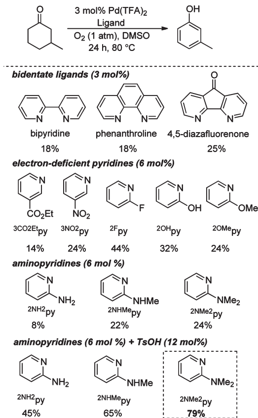
CHART 4. Ligand Effects for Aerobic Dehydrogenation of 3-Methyl Cyclohexanone
