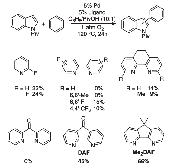
CHART 3. Identification of a Ligand for Aerobic Pd-Catalyzed Indole-Arene Cross-Coupling
