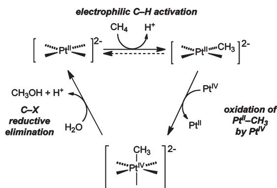
SCHEME 1. Proposed Catalytic Mechanism of the Shilov Reaction
