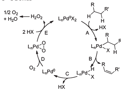
SCHEME 6. Proposed Mechanism for Pd II -Catalyzed Dehydrogenation of Saturated C–C Bonds
