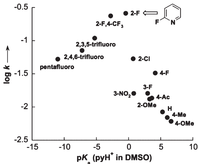
FIGURE 3. Dependence of the rate of o -xylene homocoupling on the identity of the ancillary pyridine ligands. The pK a values correspond to those for the pyridinium ions in DMSO.
