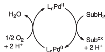
SCHEME 2. Simplified Catalytic Cycle for \text{Pd}^{\text{II}}/\text{Pd}^0 -Catalyzed Aerobic Oxidation Reactions
