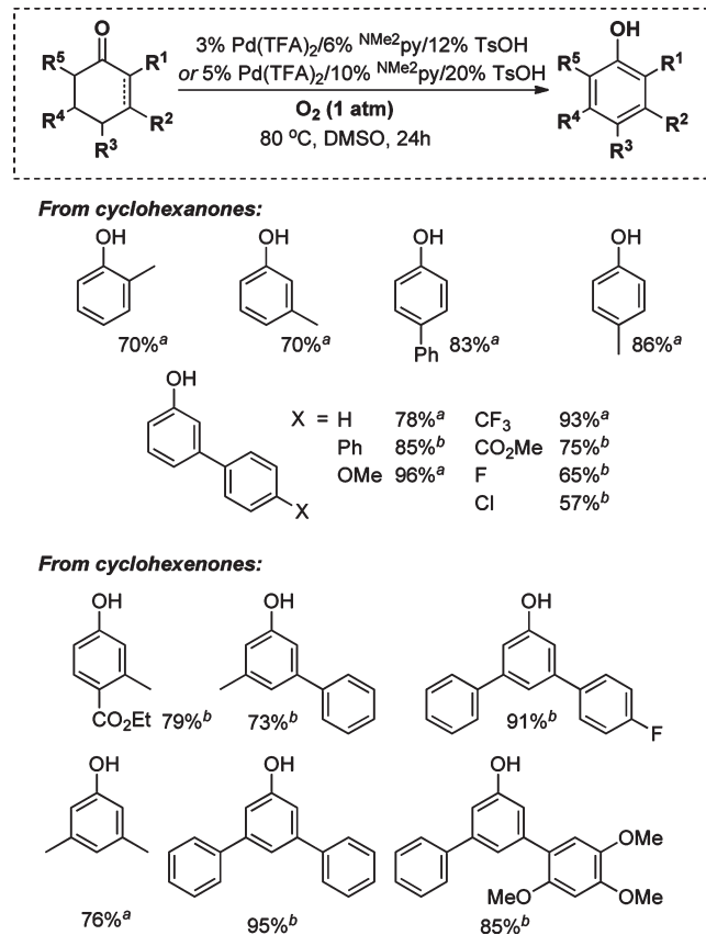
CHART 5. Phenols Prepared via Dehydrogenation of Cyclohexanone or Cyclohexenone Derivatives
