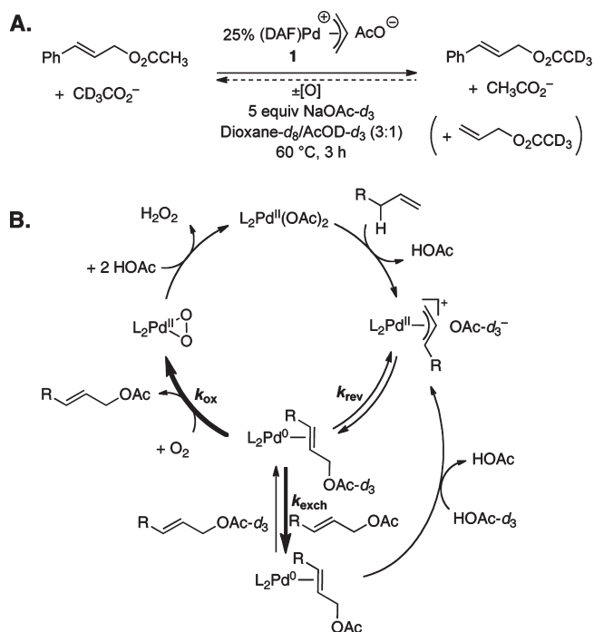
FIGURE 2. Evidence for reversible C–O reductive elimination from (DAF)Pd( \eta^3 -allyl) complexes (A), and mechanistic rationale for (L)Pd( \eta^3 -allyl)-catalyzed acetate exchange in cinnamyl acetate and the influence of an oxidant on the extent of exchange (B).
