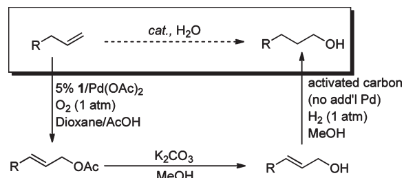
SCHEME 4. Net Anti-Markovnikov Hydration of Terminal Alkenes Involving Aerobic Allylic Acetoxylation, Acetate Cleavage, Alkene Hydrogenation Sequence
