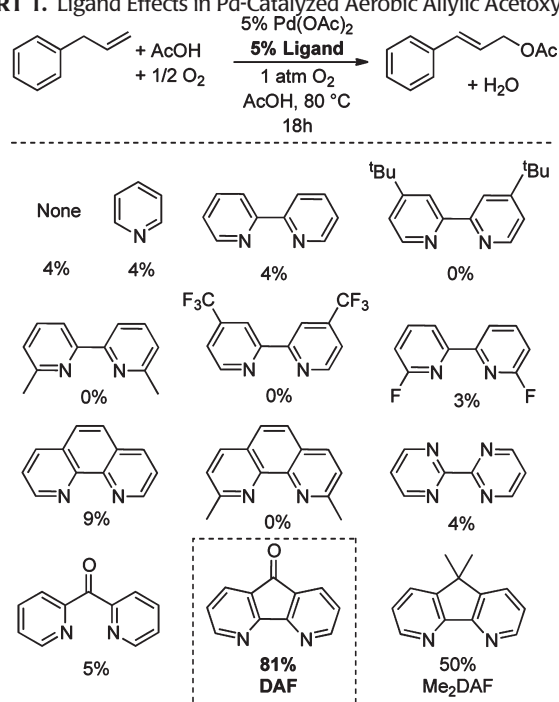
CHART 1. Ligand Effects in Pd-Catalyzed Aerobic Allylic Acetoxylation
